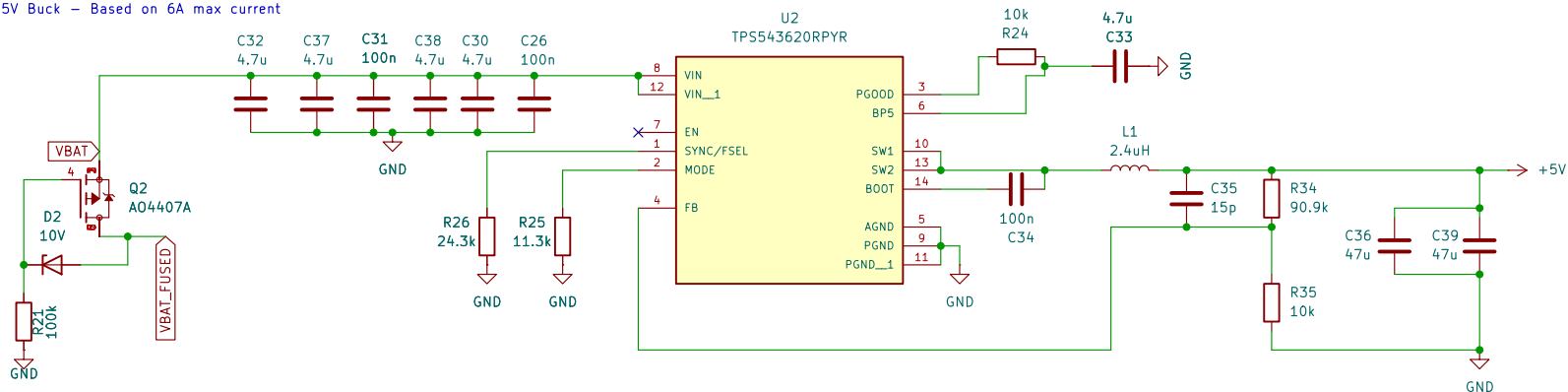
5V Buck - Based on 6A max current
