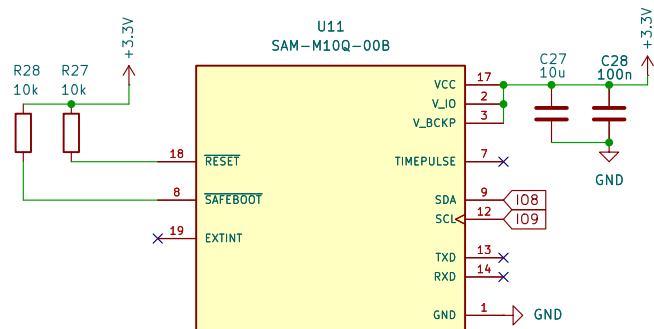
GPS Unit SAM-M10Q-00B
