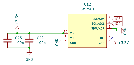
Barometer BMP581
