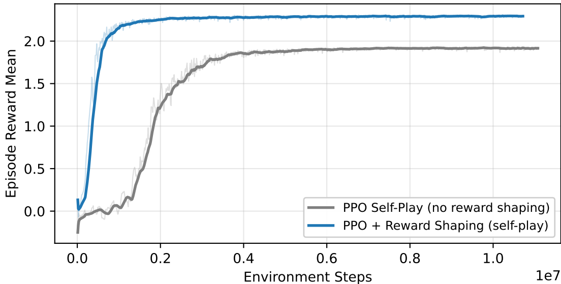
Training Curves: Effect of Reward Shaping
