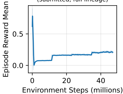
Agent 2: Reward Shaping + 70/30 (submitted, full lineage)
