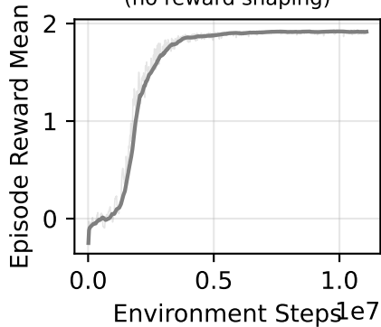
Agent 1: PPO Self-Play (no reward shaping)
