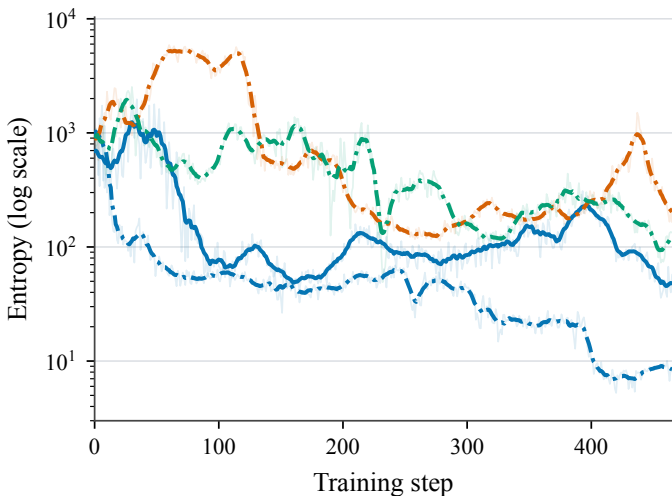
(a) Iterative self-distillation
