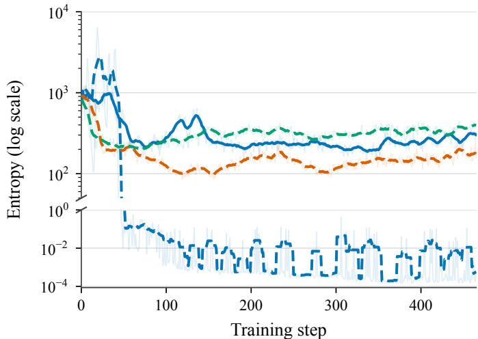
(b) Reversed iterative self-distillation
