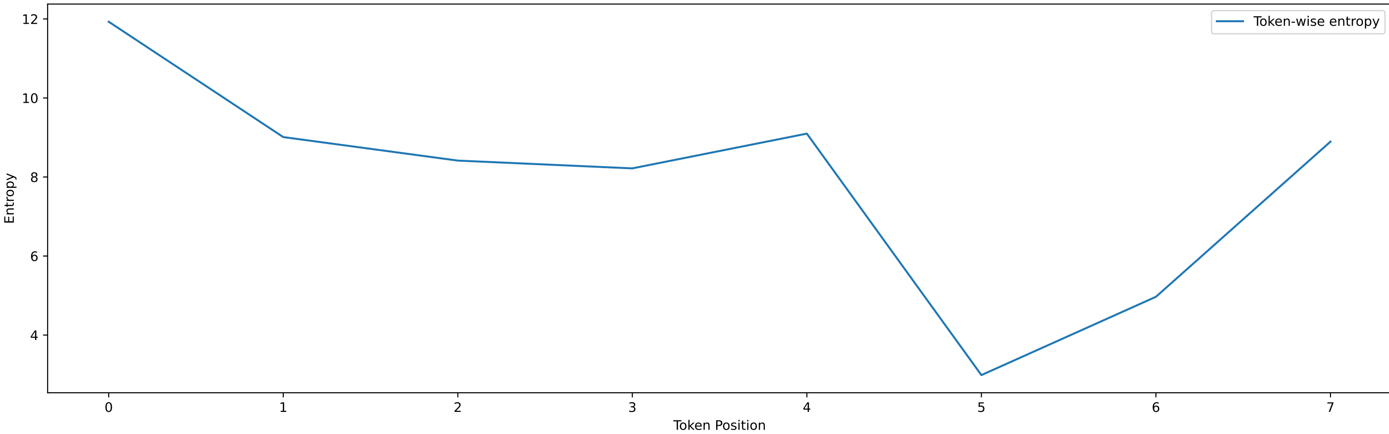
Output Text - Overall Entropy Distribution
