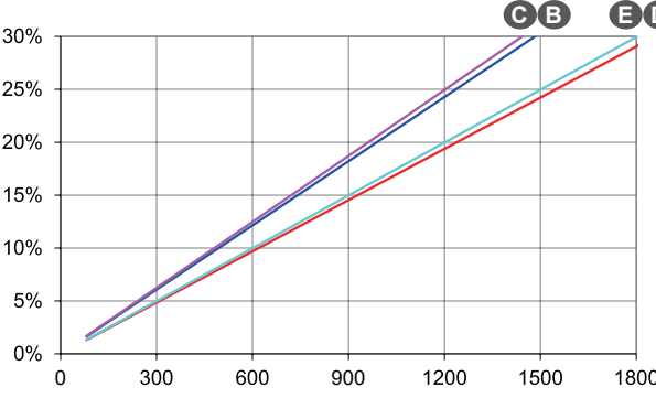
负载突卸 ((AREP+/PMG) - kVA at 0.8 P.F.
