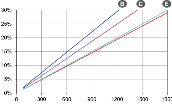
负载突卸 (SHUNT) - kVA at 0.8 P.F.
