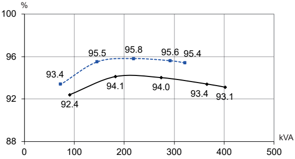
TAL-A46-H - 400V 50Hz
