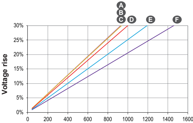
负载突卸 (AREP+/PMG)- kVA at 0.8 P.F.
