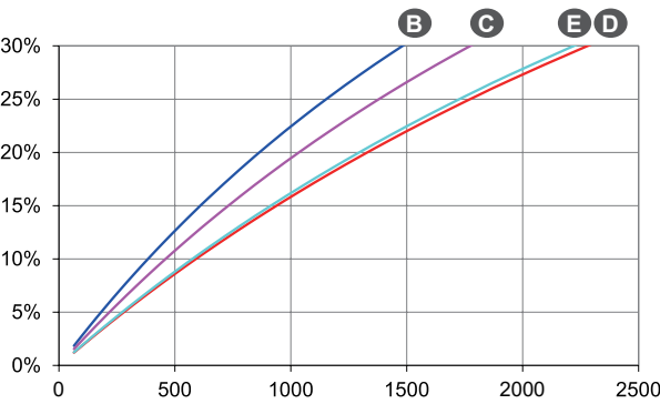
负载突加 (SHUNT) - kVA at 0.8 P.F.
