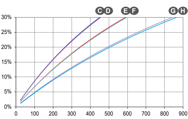
负载突加 (SHUNT) - kVA at 0.8 P.F.
