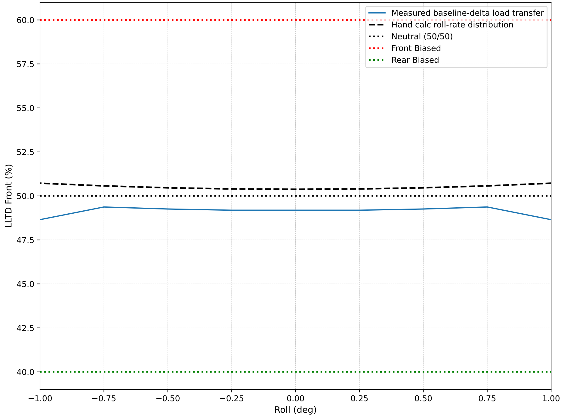
Load-Transfer LLTD vs Roll: Measured vs Roll-Rate Distribution
