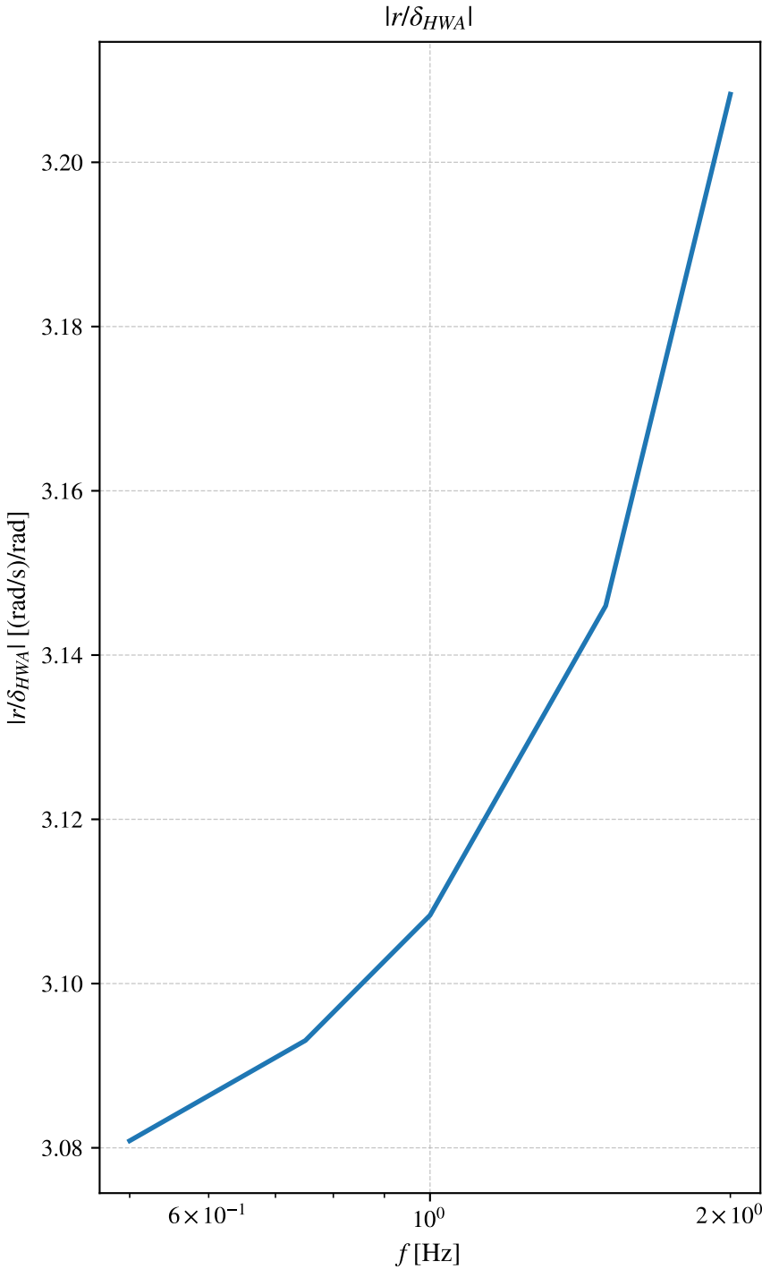
Frequency Response — Gain (ISO7401)
