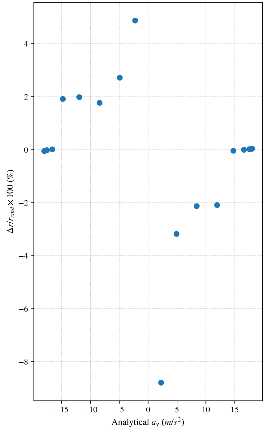
Radius Tracking Error
