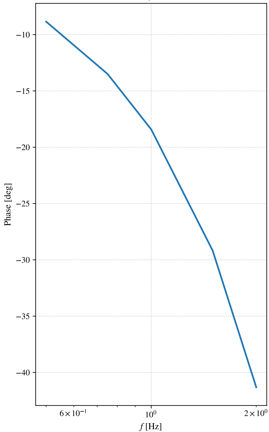
Phase: a_y vs \delta_{HWA}
