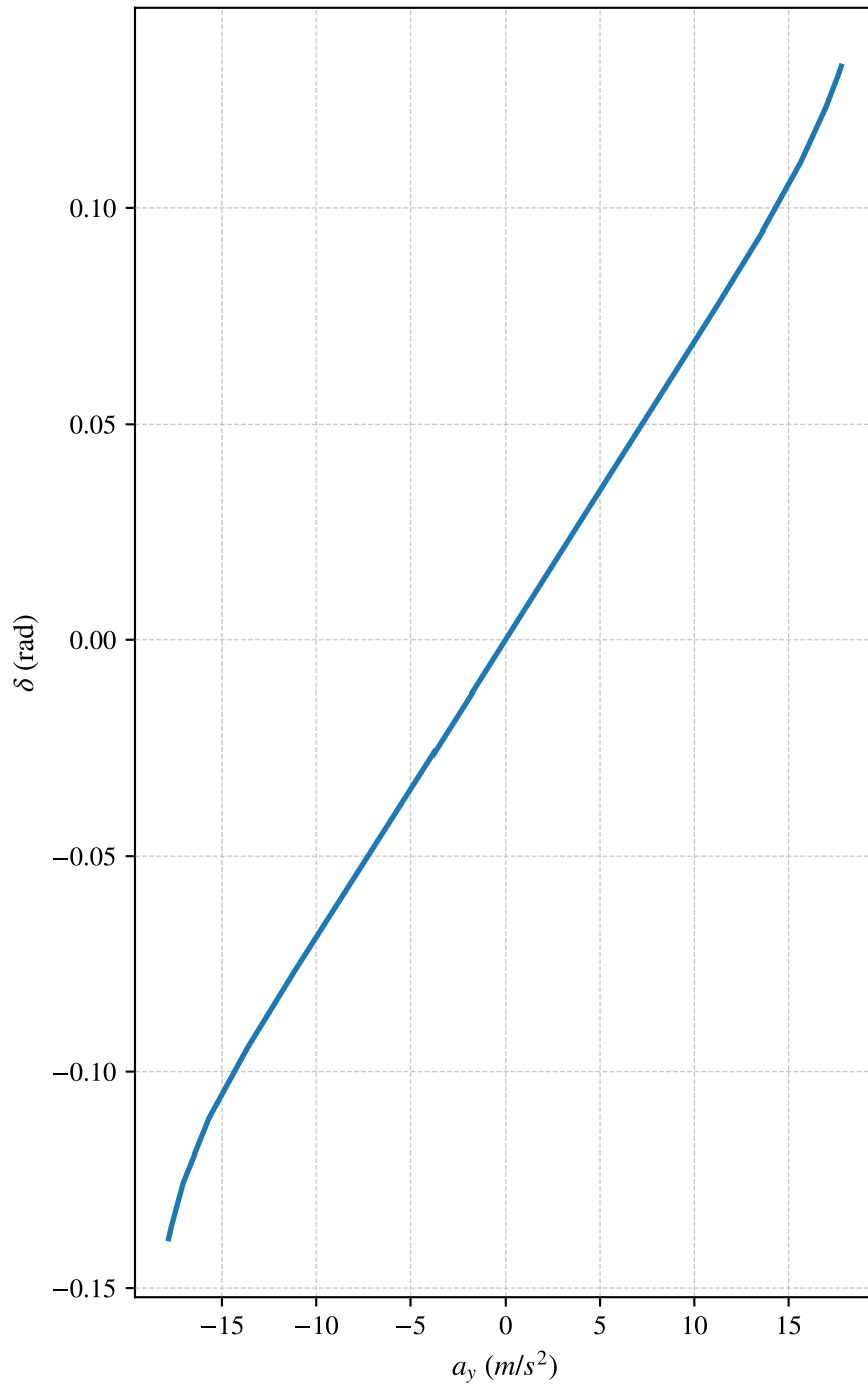
Roadwheel Angle \delta
