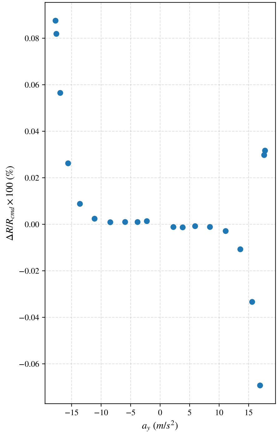
Radius Tracking Error (with v = 15 m/s)
