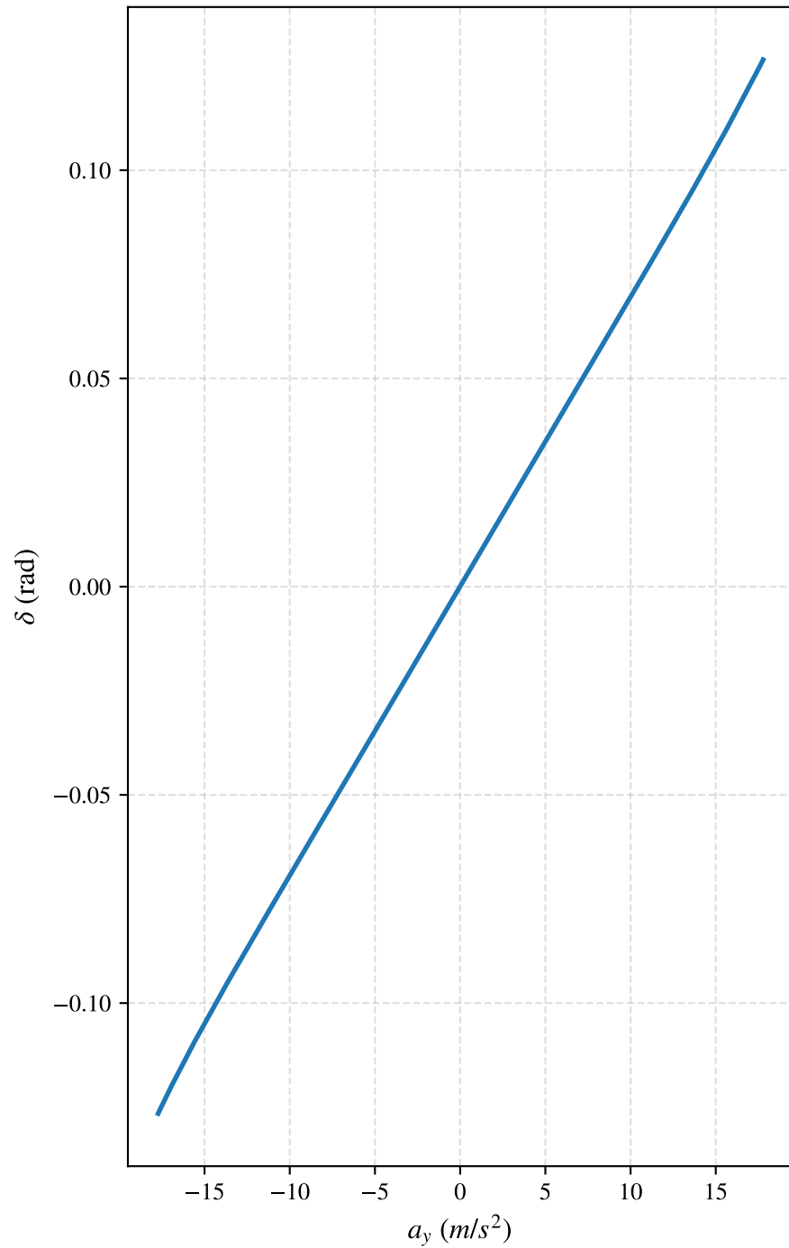
Roadwheel Angle \delta
