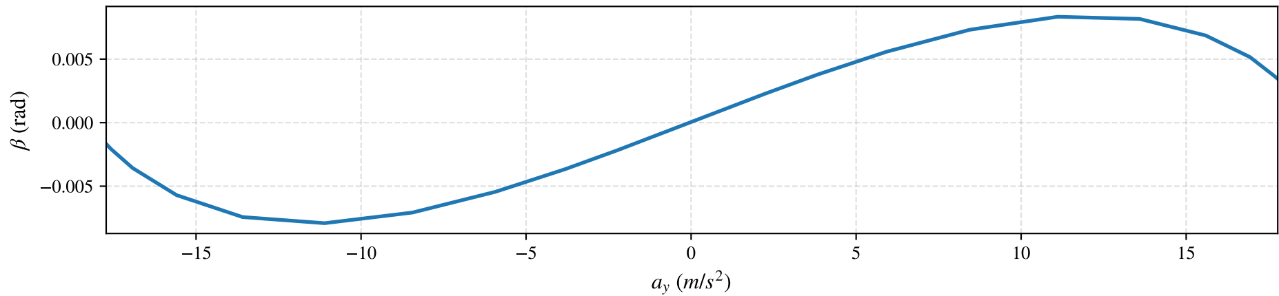
Sideslip \beta
