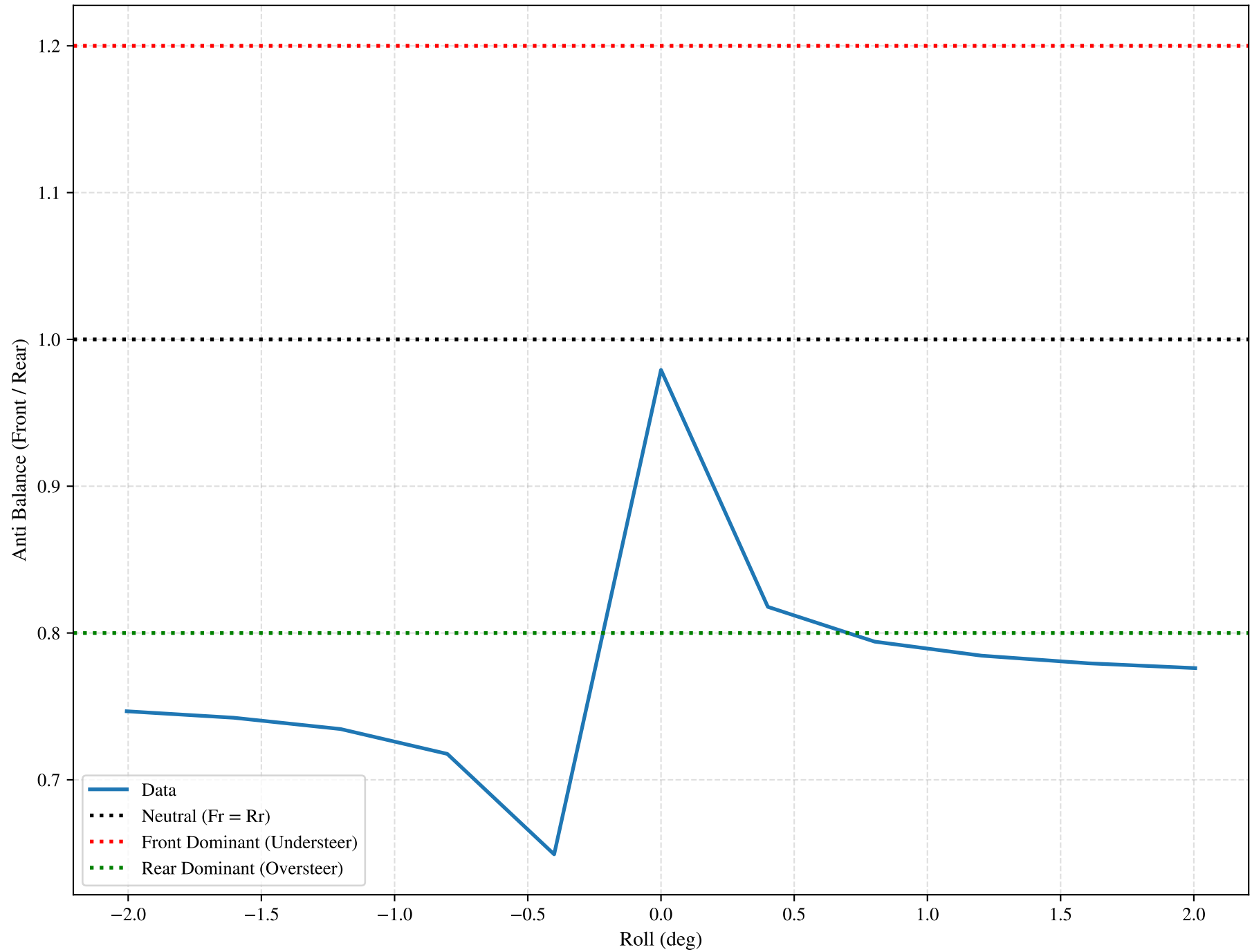
Anti Balance vs Roll
