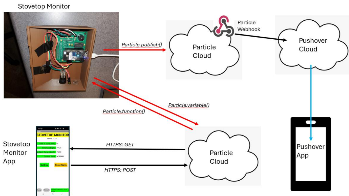
Figure 1. Stovetop Monitor System Overview.
