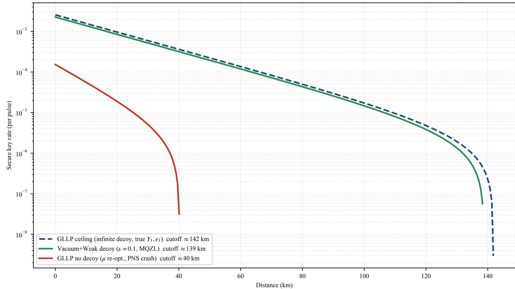
BB84 Pair 1: PNS attack — decoy recovery vs no-decoy crash (GYS params, q=0.5 , f=1.22 )
