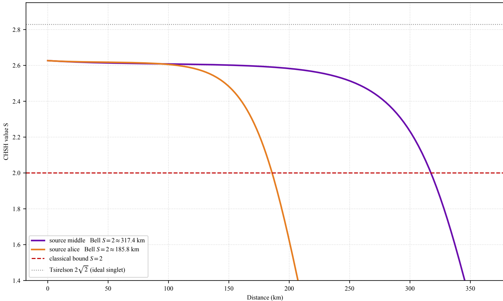
E91 as S(L): CHSH value vs distance (native MFL params, fixed \mu ) both source placements; S=2 is a Bell cutoff, NOT a key-rate cutoff
