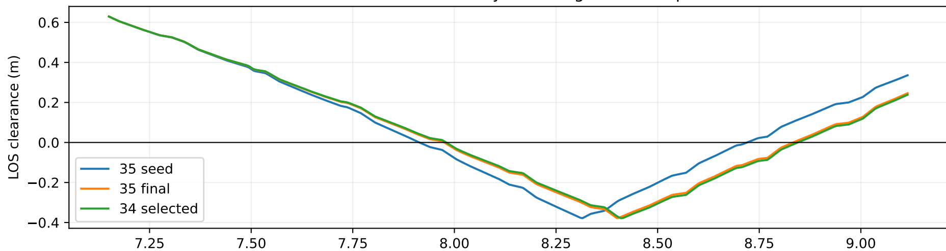
B: post-solve LOS correction breaks a PVA-safe solution
