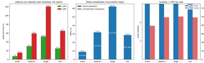
Fig. 4. Test C: latency and delay breakdown per size class. Small is served fast in isolation but is penalised \sim 1.4 \times inside the mixed queue; all classes complete with zero errors on six fixed pods.
