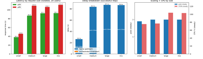
Fig. 4. Test C: latency and delay breakdown per size class. Small is served fast in isolation but is penalised 3.5\times inside the mixed queue.
