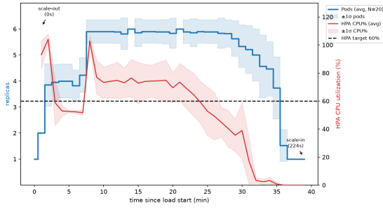
Fig. 1. Test A: pod replicas and CPU% against time ( N=20 average with \pm 1\sigma band). The sawtooth scales out 1 \rightarrow 2 \rightarrow 4 \rightarrow 6 under the ramp and steps back down 6 \rightarrow 5 \rightarrow 4 \rightarrow 3 \rightarrow 2 \rightarrow 1 during the valleys.
