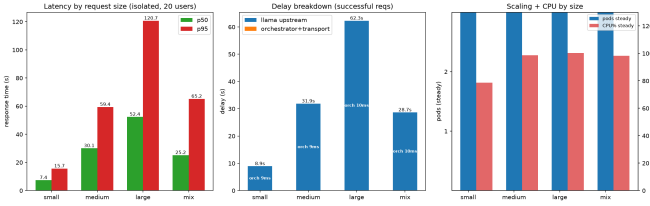
Fig. 4. Test C: latency and delay breakdown per size class. Small is served fast in isolation but is penalised 1.4\times inside the mixed queue; all classes complete with zero errors on six fixed pods.
