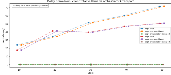
Fig. 3. Delay split (total / upstream / orchestrator) per level. The orchestrator share is \approx 11 ms; llama decode dominates. A small x-position jitter ( \pm 0.6 users) is applied so the overlapping total and upstream lines remain separately visible.
