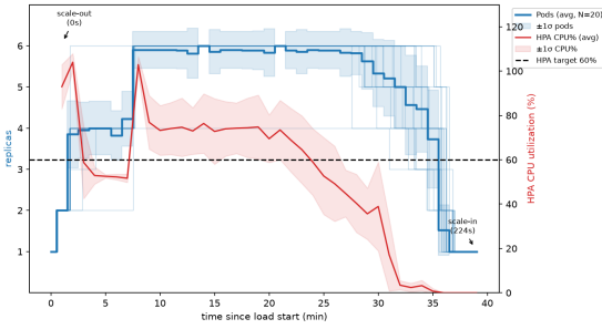
Fig. 1. Test A: pod replicas and CPU% against time ( N=20 ). Thin lines are individual runs; the bold line is the average. The sawtooth scales out 1→2→4→6 under the ramp and steps back down 6→5→4→3→2→1 during the valleys.
