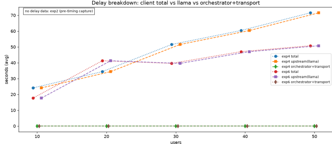
Fig. 3. Delay split (total / upstream / orchestrator) per level. The orchestrator share is \approx 11 ms; llama decode dominates. A small x -position jitter ( \pm 0.6 users) is applied so the overlapping total and upstream lines remain separately visible.
