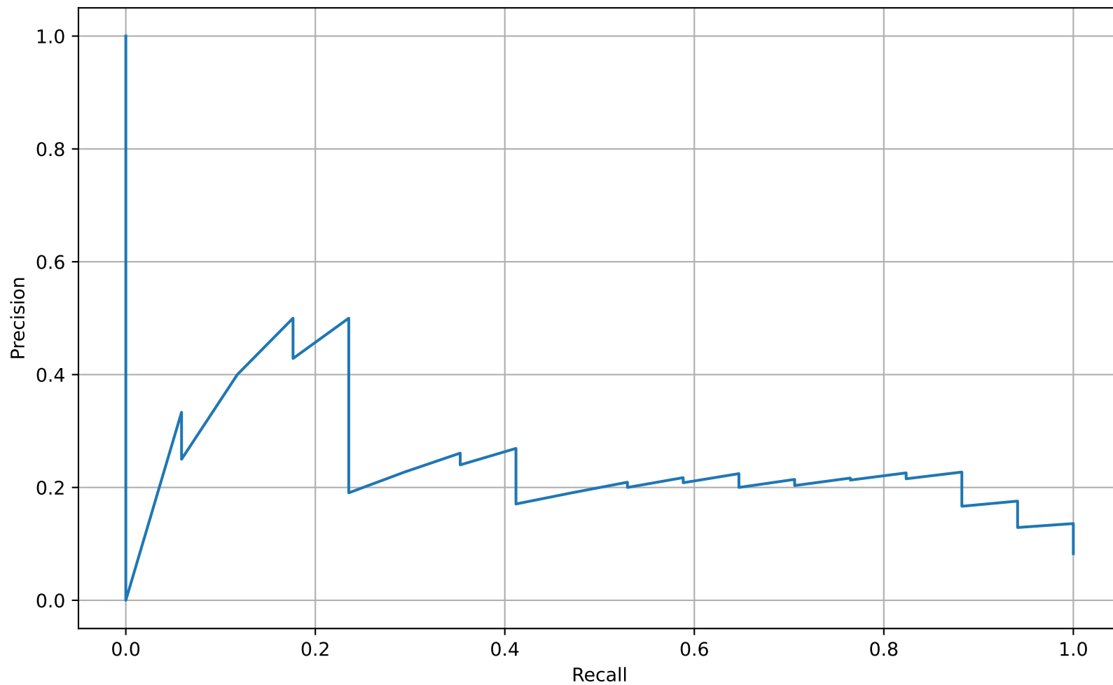
Precision-Recall Curve
