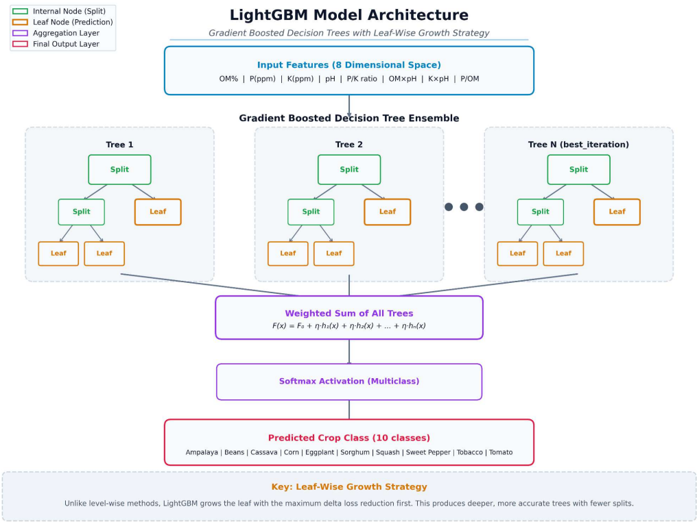
Figure 3.24 LightGBM Model Architecture used in the TANIM system
