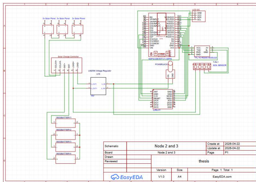
Node 2 and 3 Transmitter Schematic Diagram
