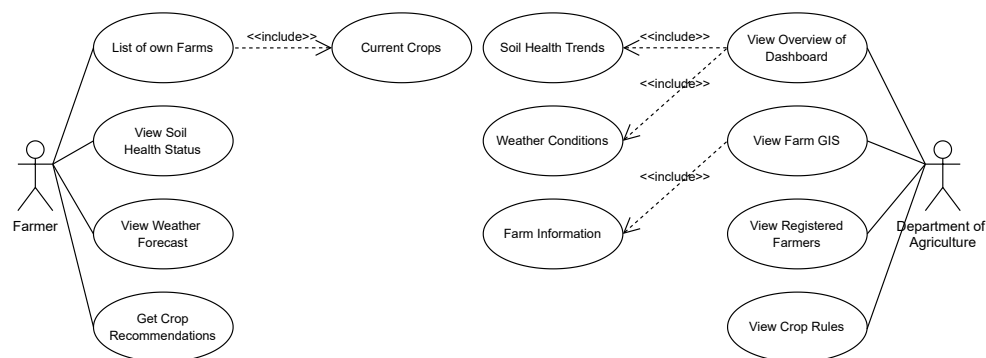
Figure 3.15 Use Case Diagram
