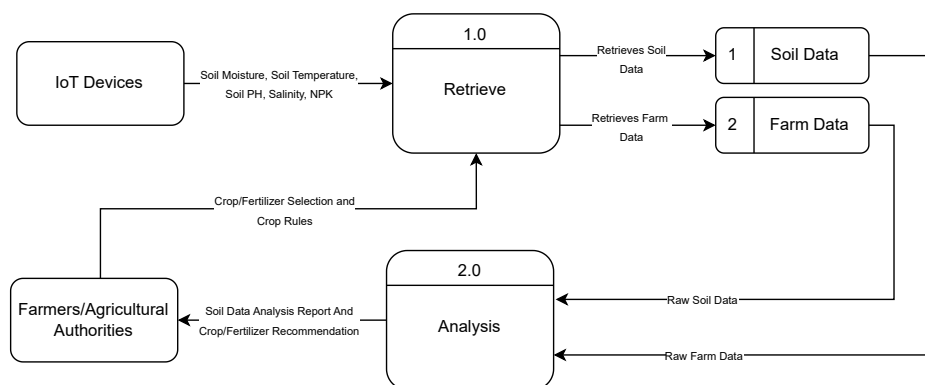
Figure 3.9 Data Flow Diagram
