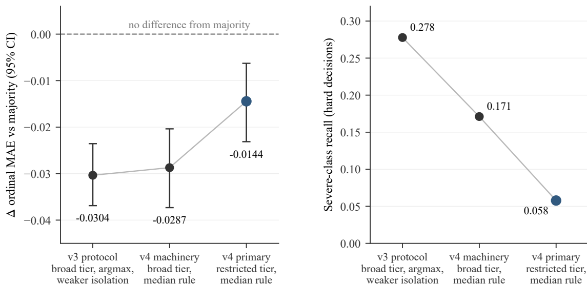
Figure 10: Effect of protocol correction on the headline result. Correction shrinks both the headline margin and severe-class hard assignment. The decision-rule change reduces severe recall with little change in ordinal error; the restricted feature tier accounts for most of the remaining attenuation. CI = confidence interval.
