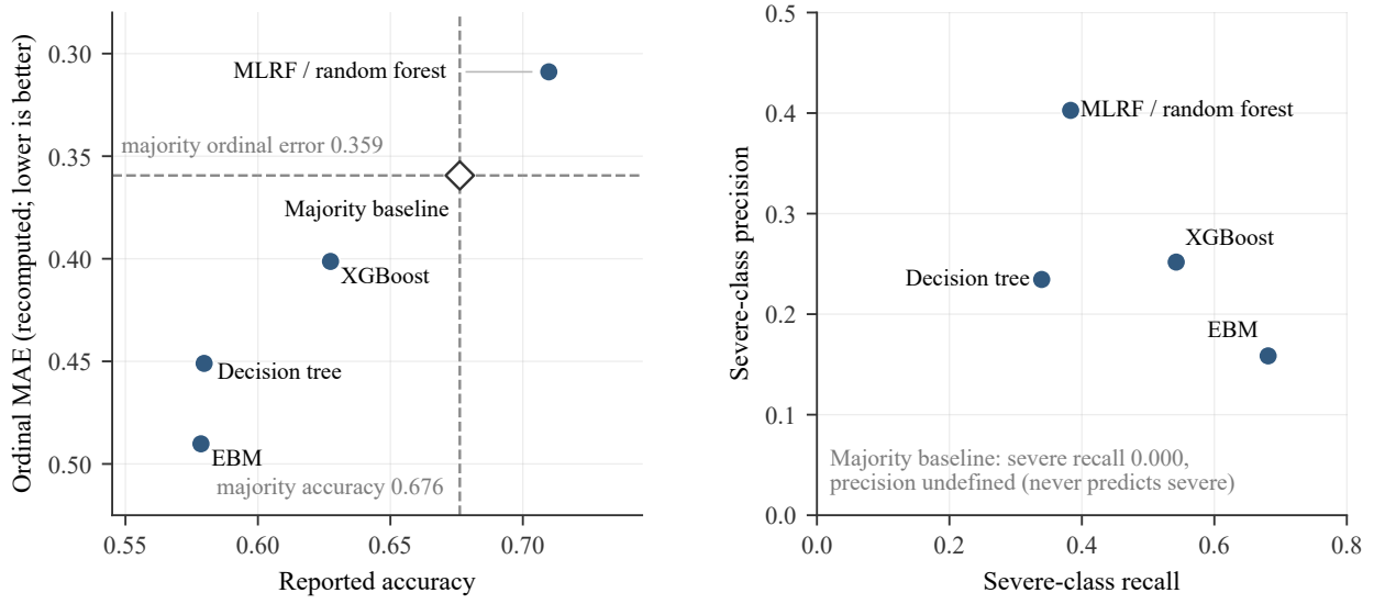
Figure 3: Re-analysis of the prior reported confusion matrices. Left: three models fall below the majority-accuracy baseline, while only the multilevel random forest (MLRF) beats the majority ordinal-error baseline. Right: the same models occupy different severe precision–recall tradeoffs.
