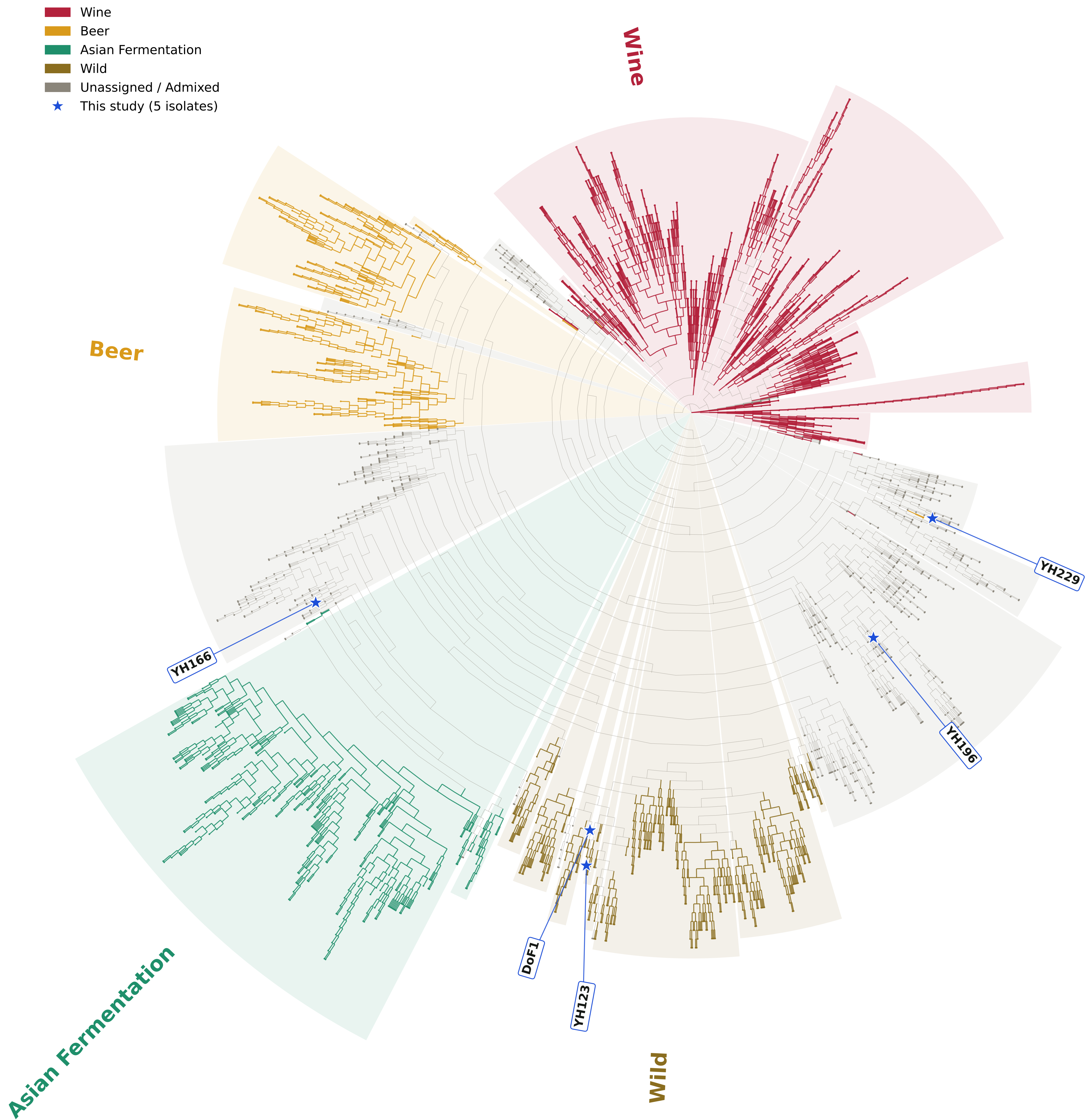
Phylogenomic placement of 5 Bloomington isolates among 3,034 S. cerevisiae genomes (Loegler et al. 2024 panel + this study; FastTree, 46,705 shared SNPs)
