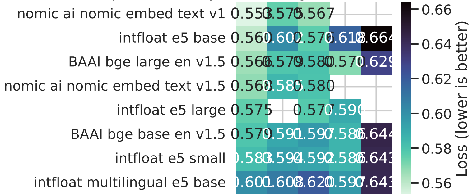
Composite Loss by Embedding Model × Chunker (min over c,o)
