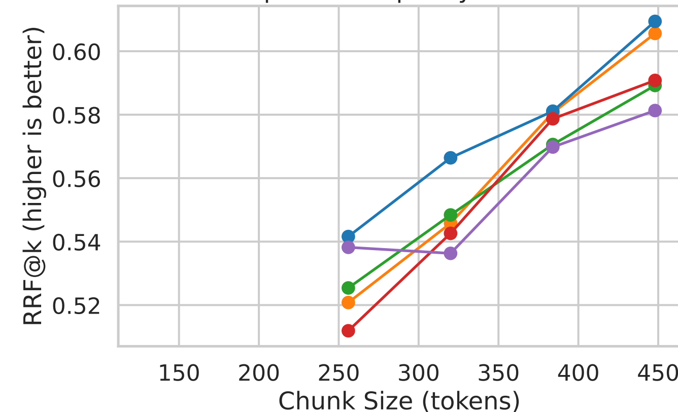
RRF@k vs Chunk Size at overlap=64 — Top 5 by mean score • RRF@k • k=10 • \beta=2
