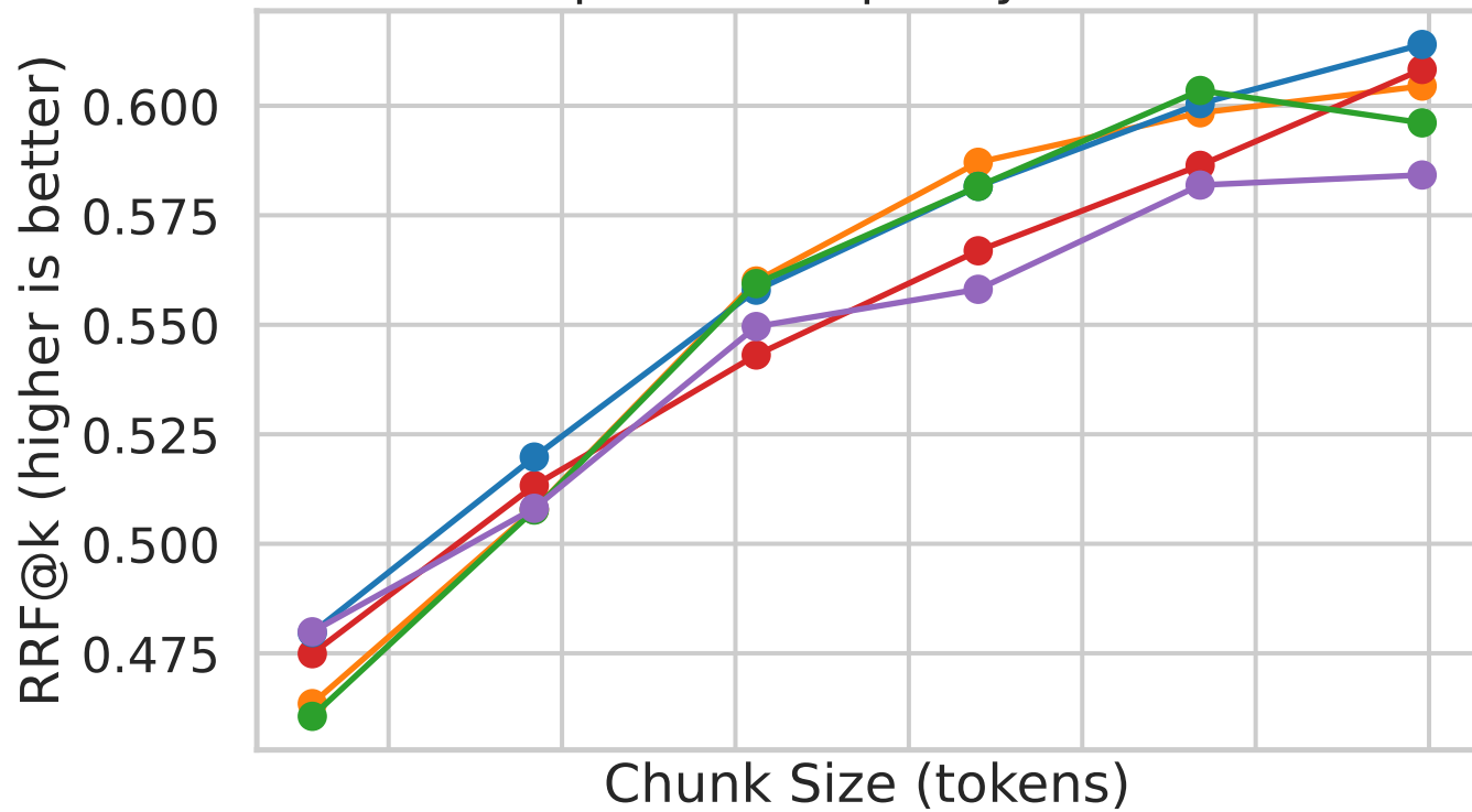
RRF@k vs Chunk Size at overlap=32 — Top 5 by mean score • RRF@k • k=10 • \beta=2
