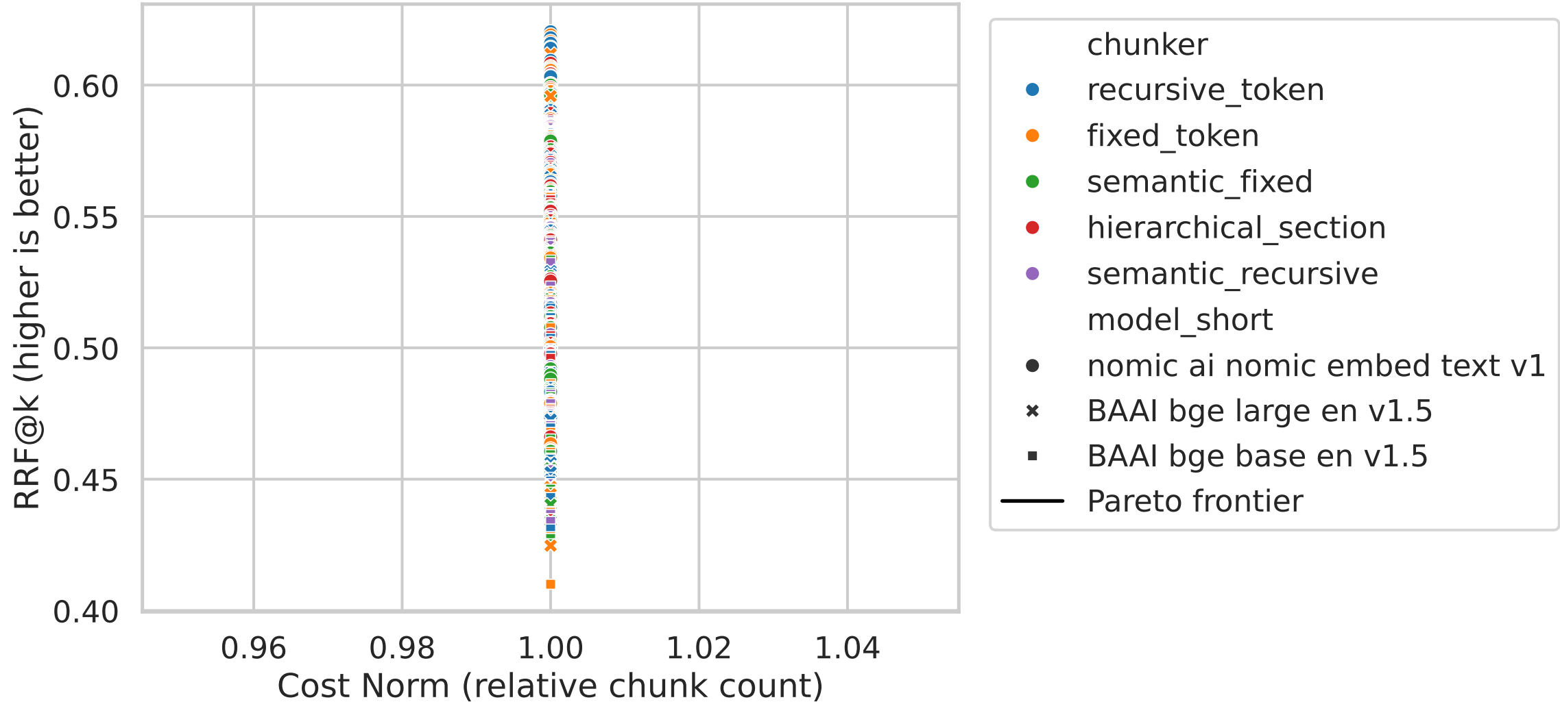
Quality-Cost Trade-off (RRF@k vs Cost Norm) • k=10 • \beta=2
