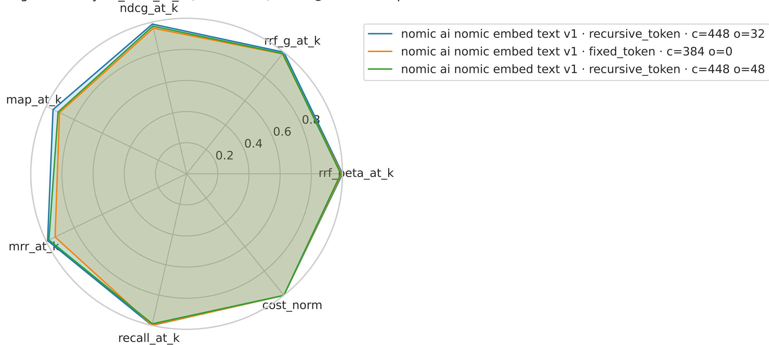
Top-3 Configurations by \text{rrf\_beta\_at\_k} (Normalized) • \text{RRF@k} • k=10 • \beta=2
