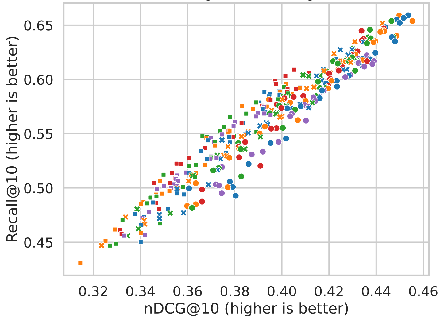
Recall@10 vs nDCG@10
