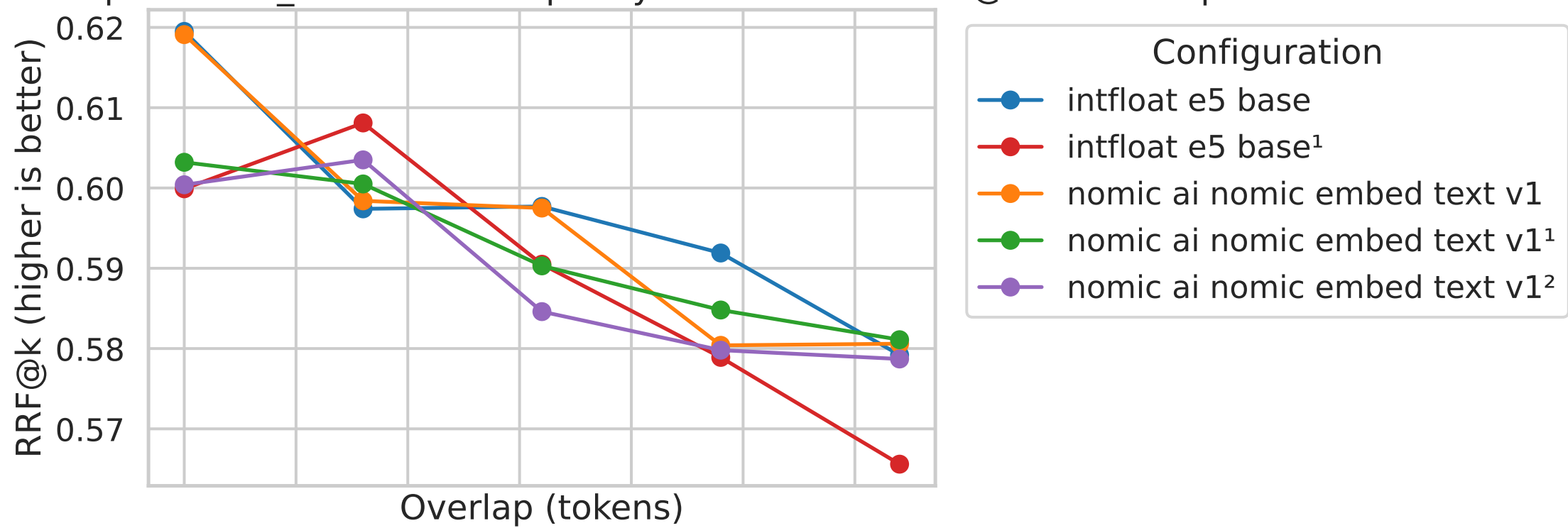
RRF@k vs Overlap at token_size=448 — Top 5 by mean score • RRF@k • k=10 • \beta=2
