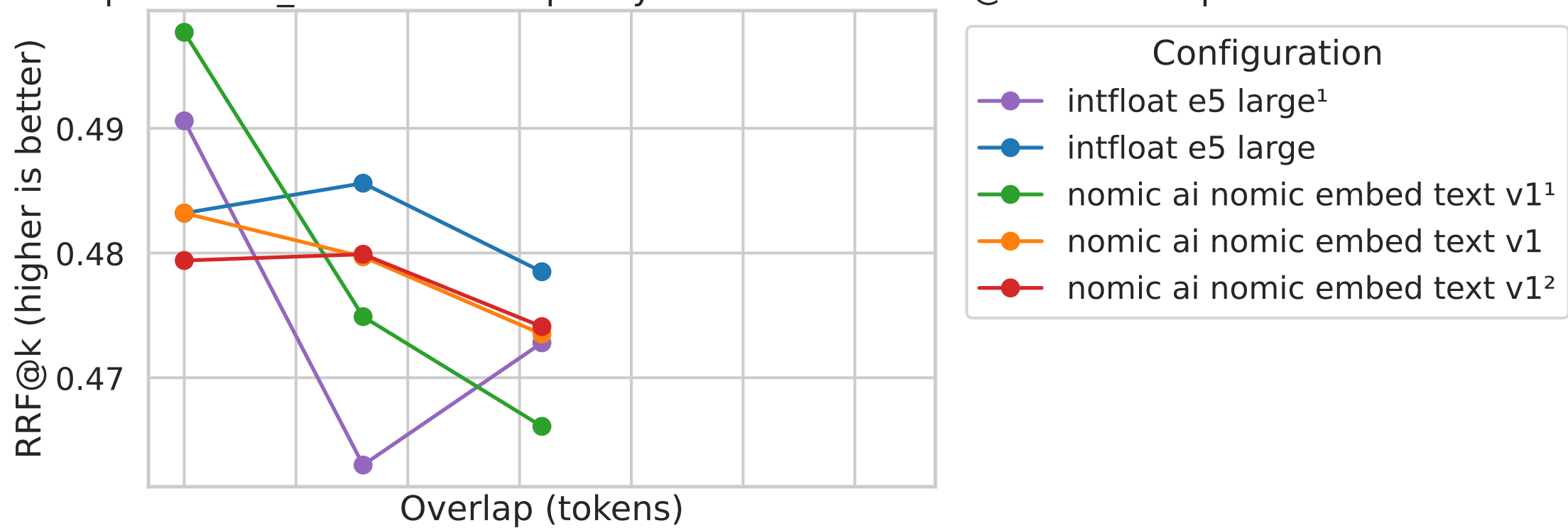
RRF@k vs Overlap at token_size=256 — Top 5 by mean score • RRF@k • k=10 • \beta=2
