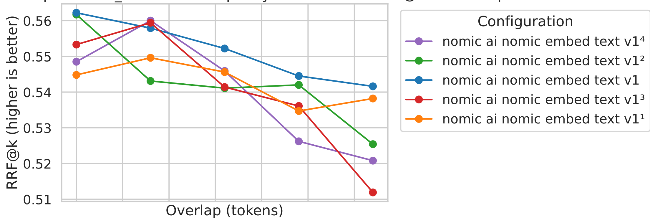
RRF@k vs Overlap at token_size=384 — Top 5 by mean score • RRF@k • k=10 • \beta=2
