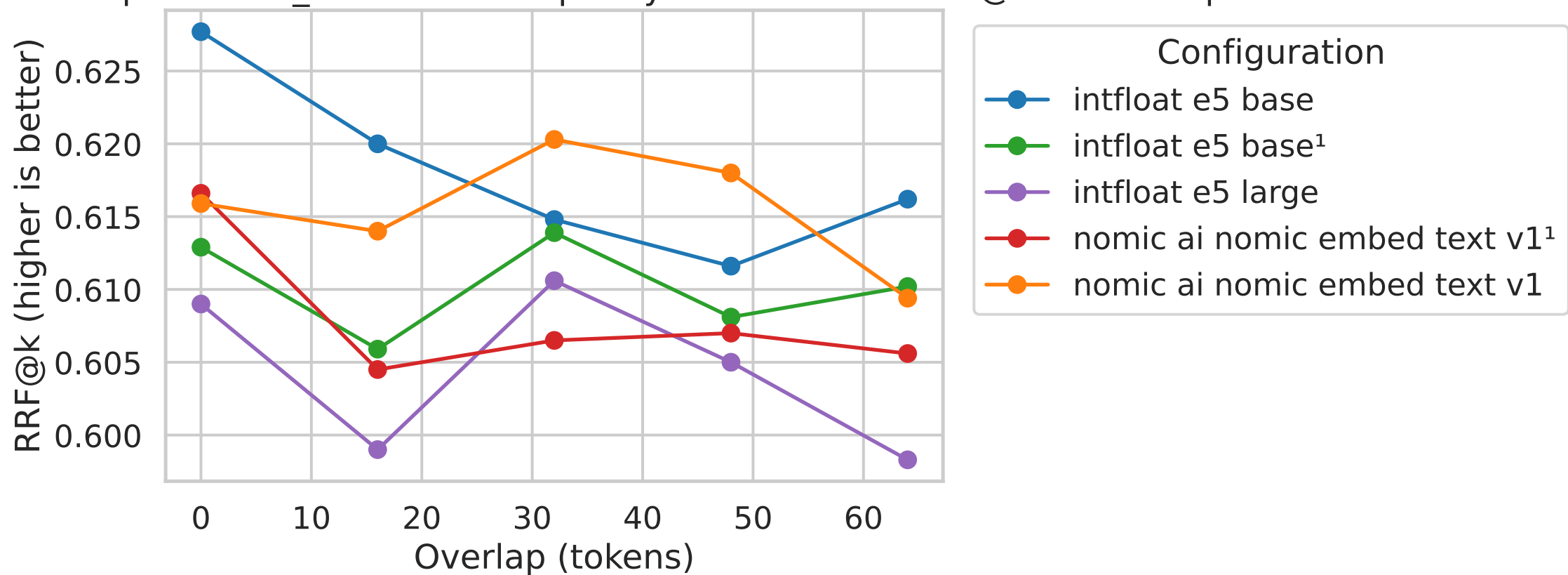
RRF@k vs Overlap at token_size=448 — Top 5 by mean score • RRF@k • k=10 • \beta=2
