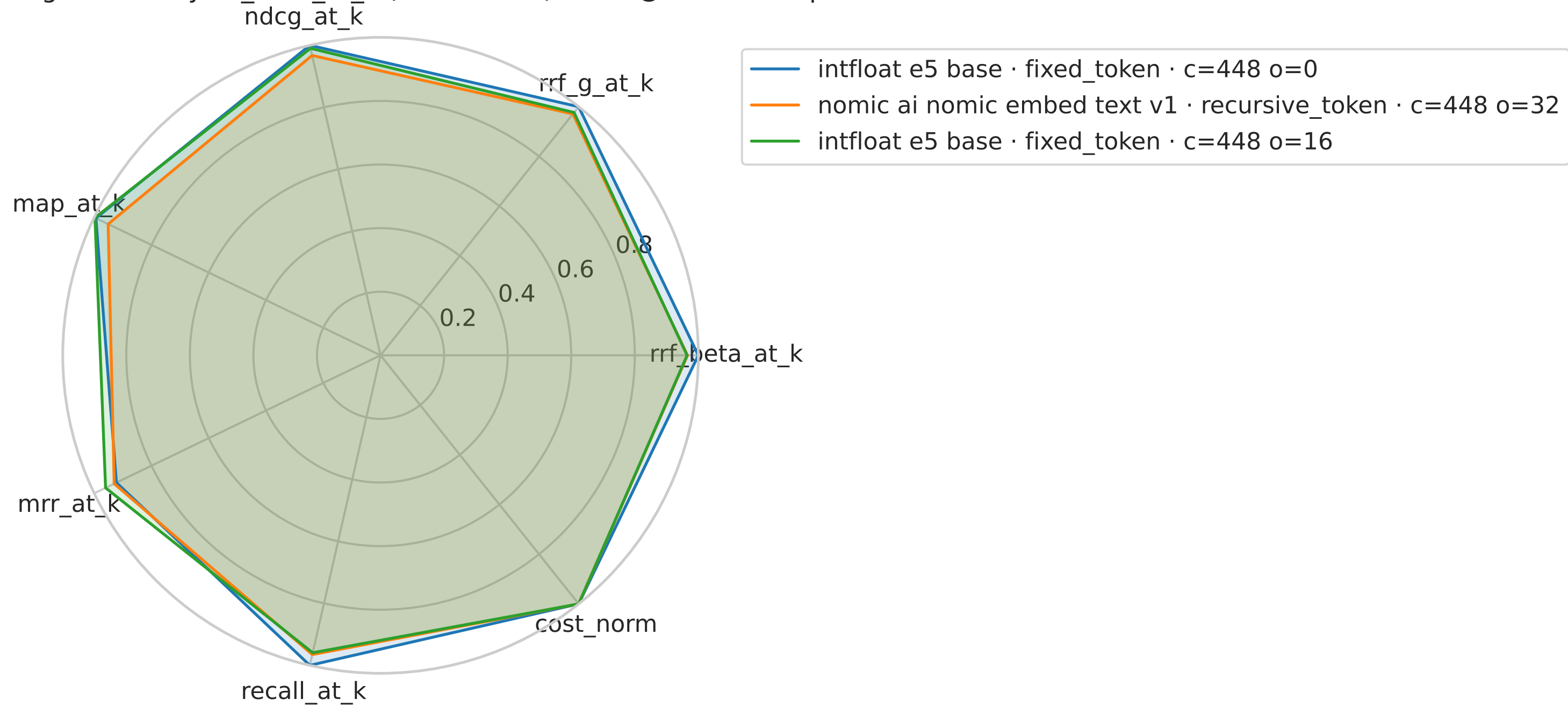
Top-3 Configurations by rrf_beta_at_k (Normalized) • RRF@k • k=10 • \beta=2
