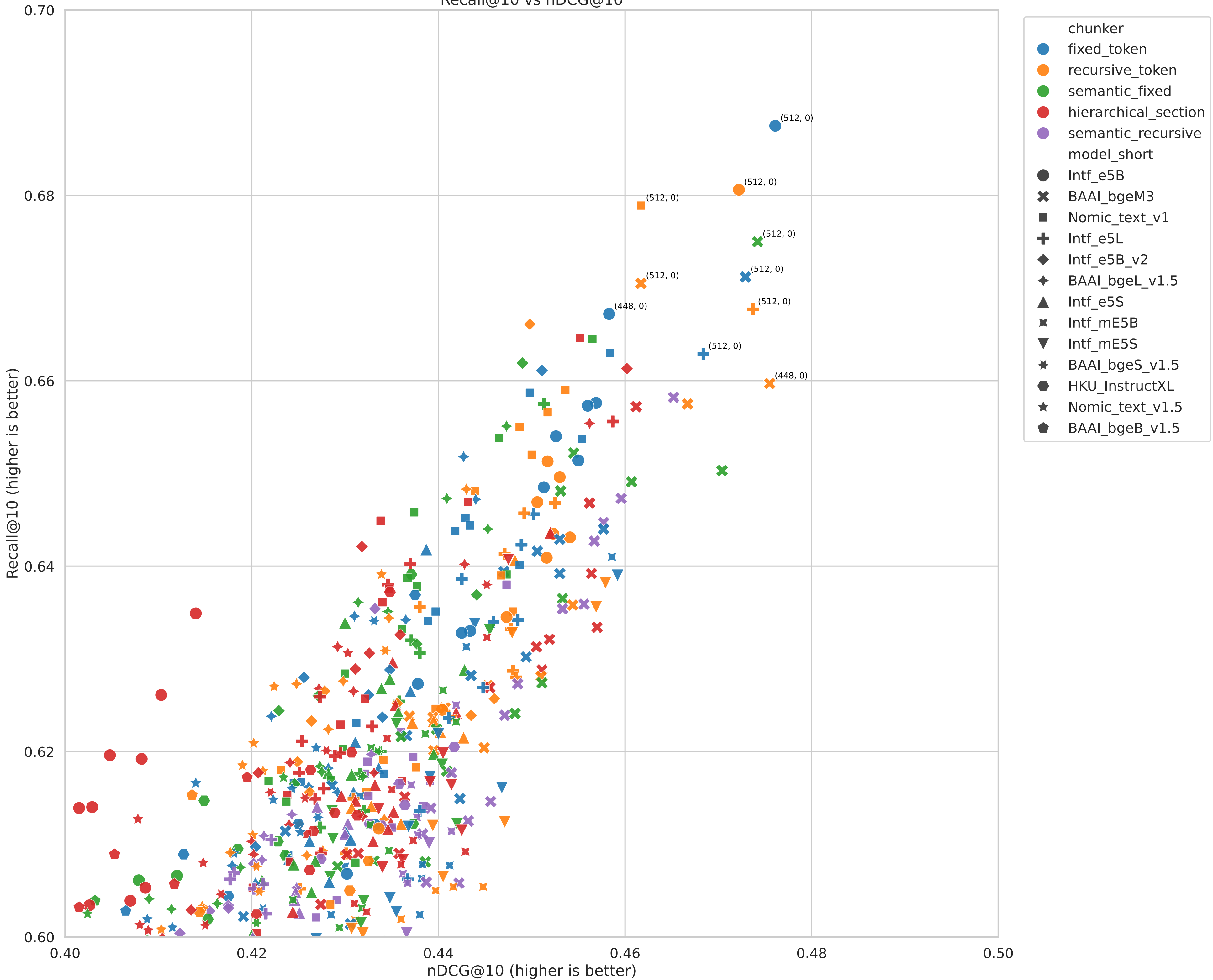
Recall@10 vs nDCG@10
