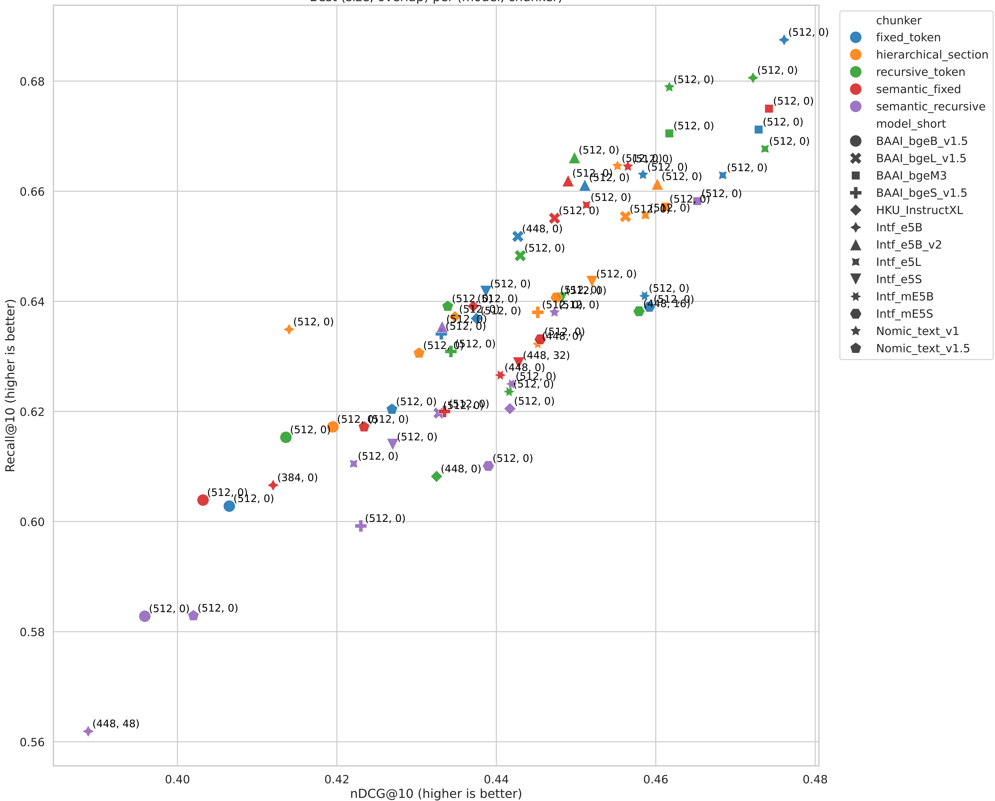
Recall@10 vs nDCG@10 Best (size, overlap) per (model, chunker)
