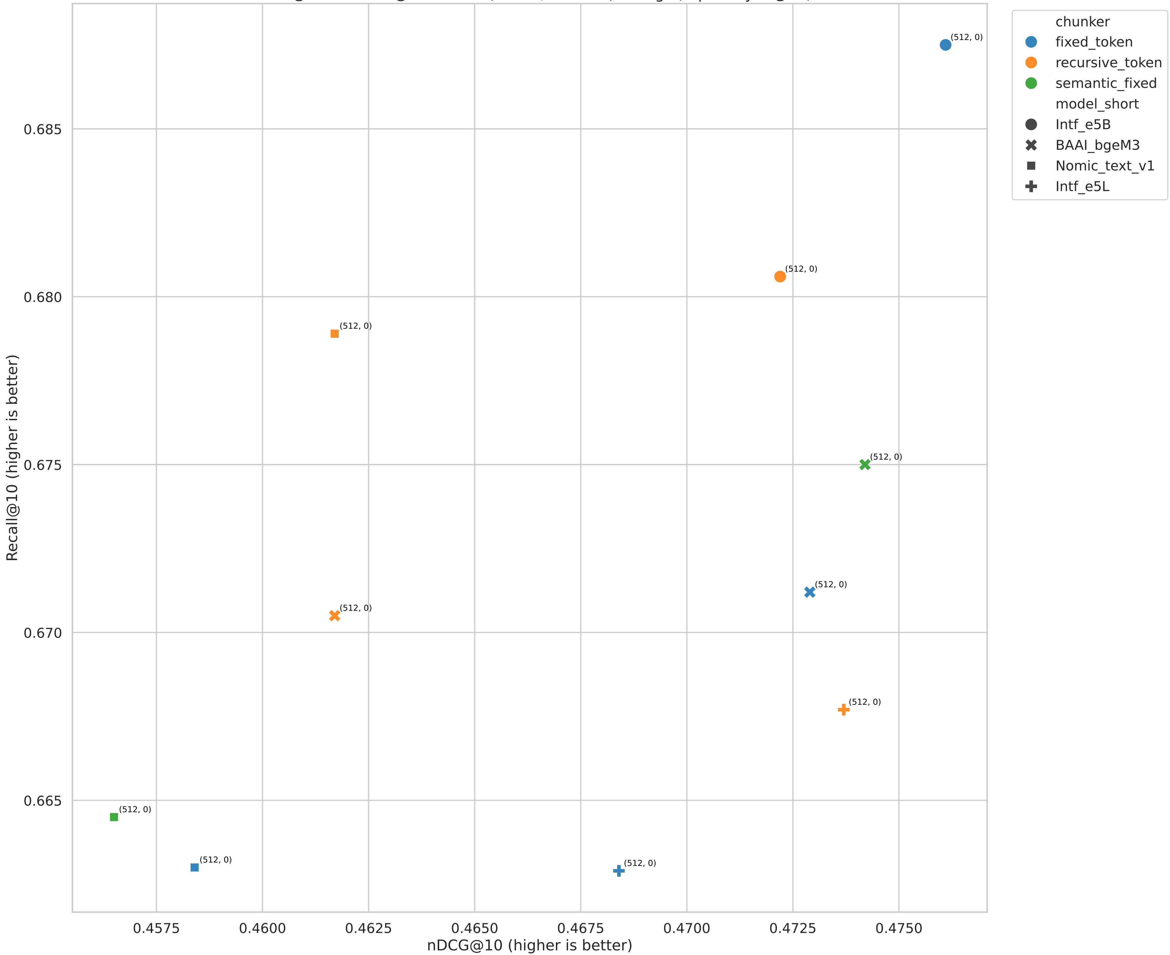
Recall@10 vs nDCG@10 — Best (model, chunker) configs (Top 10 by F 2 @10)
