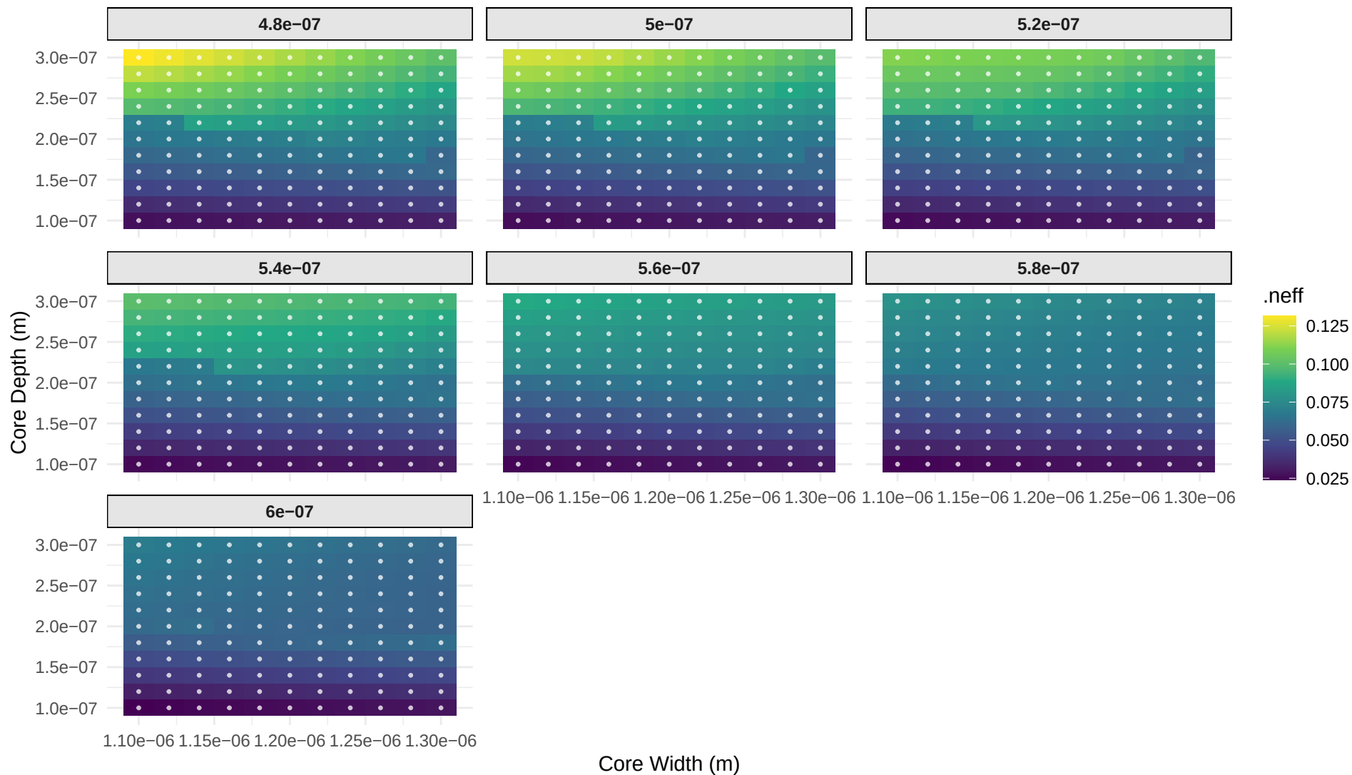
Delta Effective Index: Width vs Depth (Sliced by Gap)
