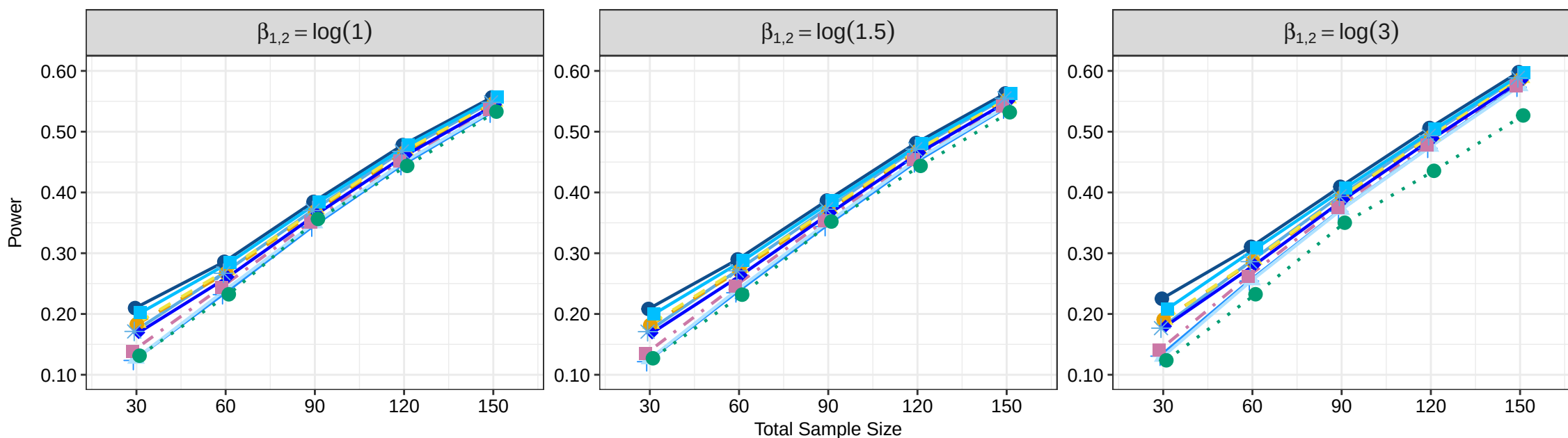
True Effect Size: \delta = 0.30
