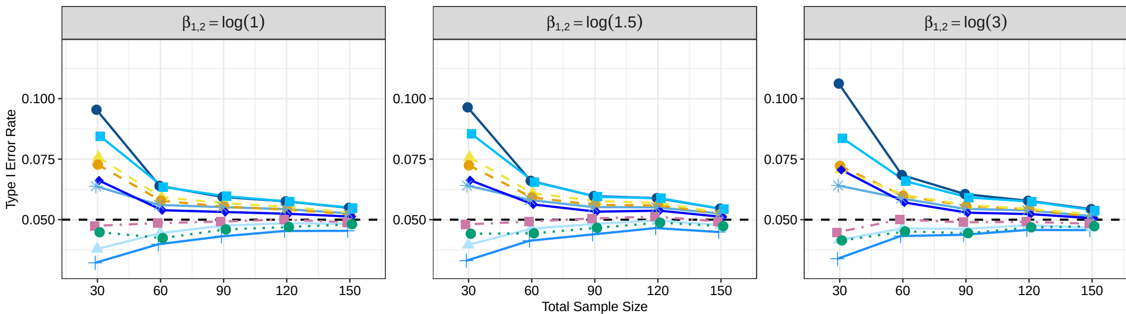
True Effect Size: \delta = 0.15
