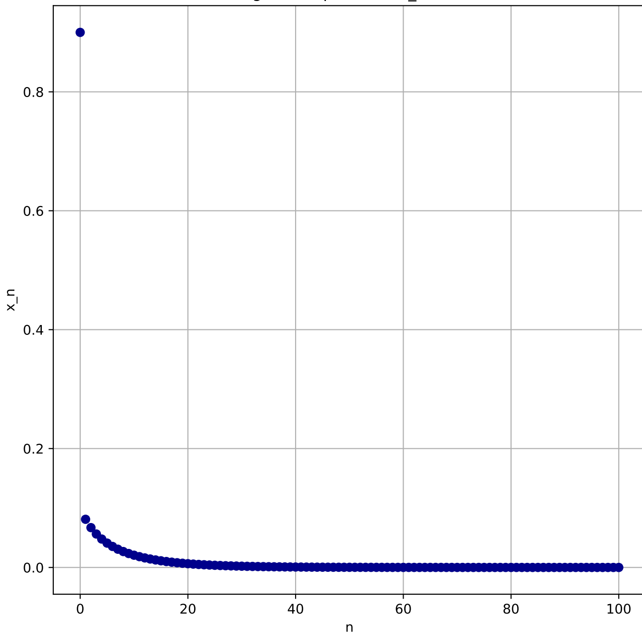
Logistic Map: r=0.9 , x_0=0.9
