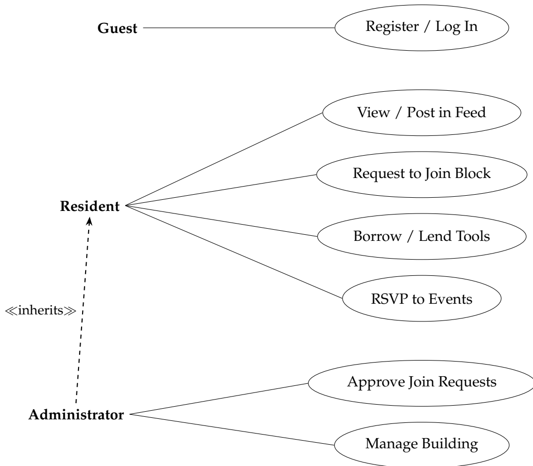
Figure 3.2: UML Use Case Diagram mapping system actors to primary functionalities.
