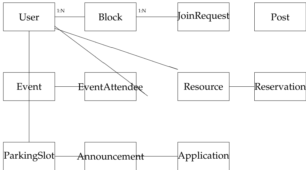
Figure 3.4: Entity-Relationship (ER) topology mapping the relational database structure of the NEST application.
