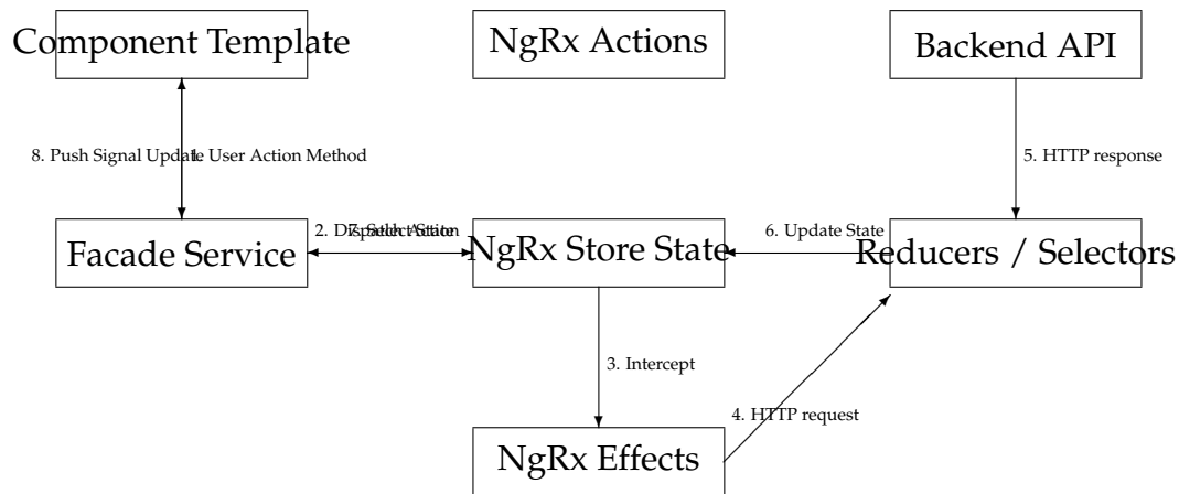
Figure 3.2: Reactive state data flow in the frontend utilizing the NgRx Facade and Signal paradigms.
