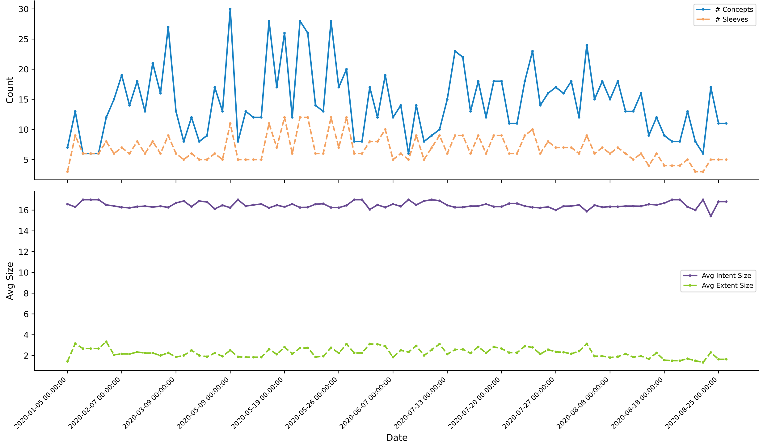
Figure 9 - Temporal Complexity
