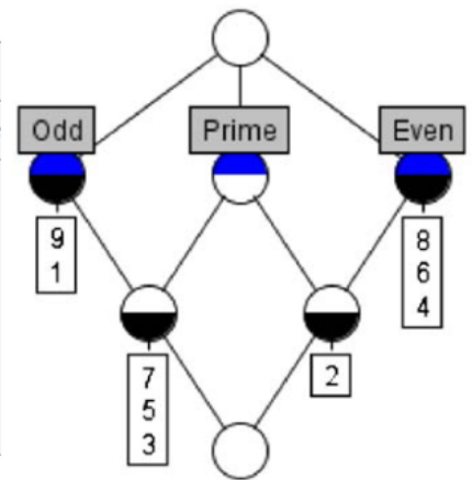
Fig. 22: Concept lattice corresponding to the formal context
