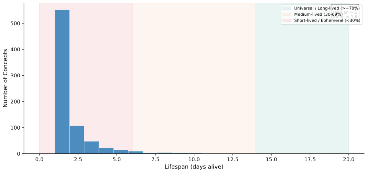
Fig. 20: TCA Concept Lifespan Distribution
