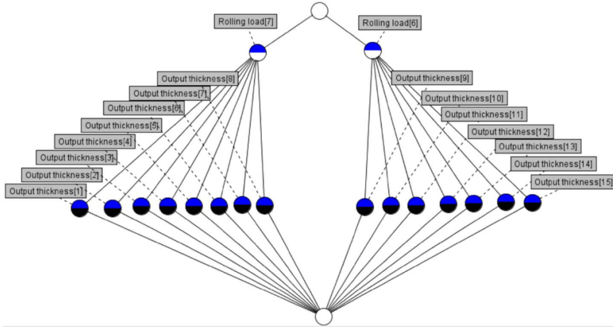
Fig. 23: Line diagram for analysis of the rolling load P and output thickness ho
