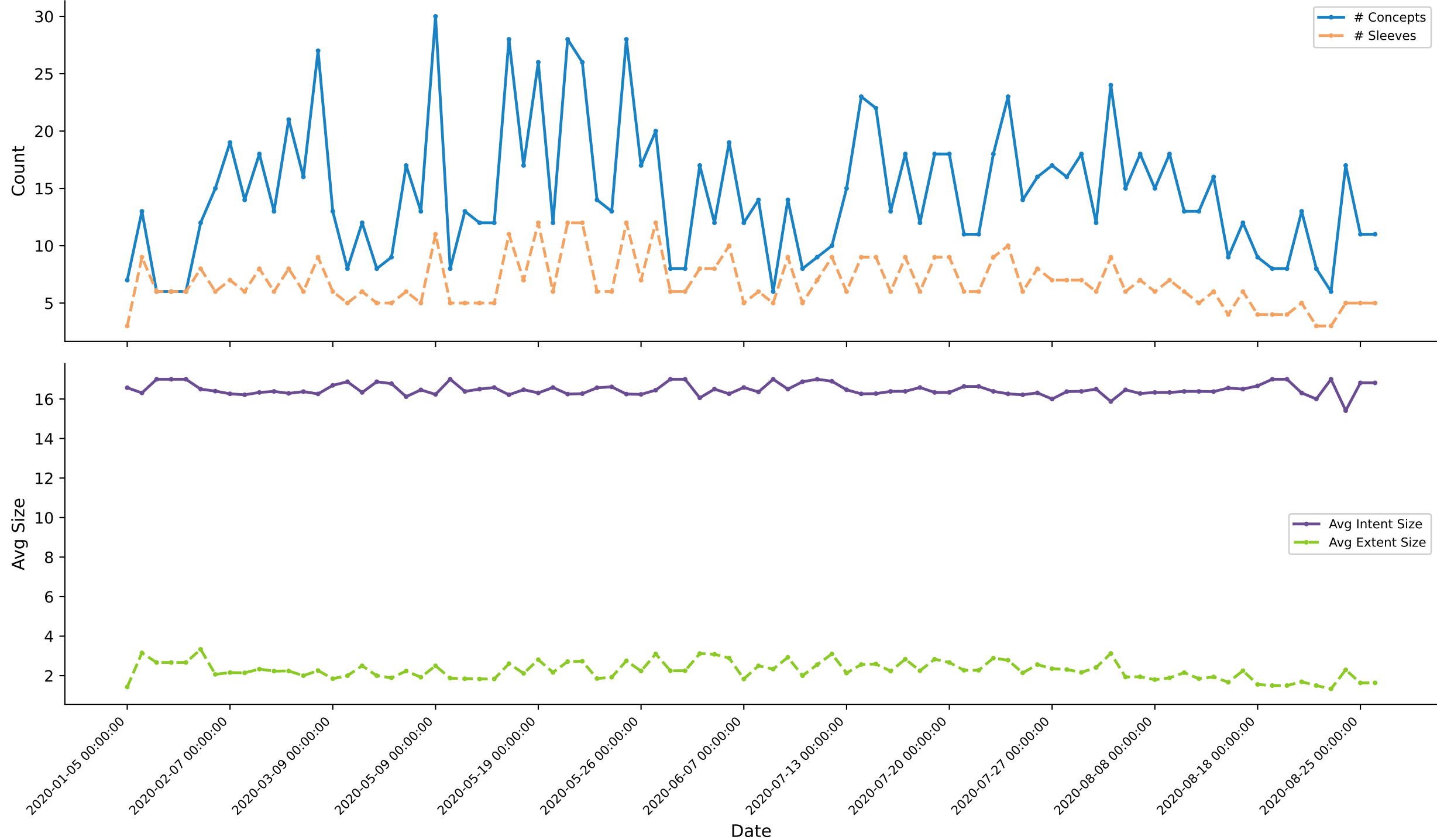
Figure 9 - Temporal Complexity
