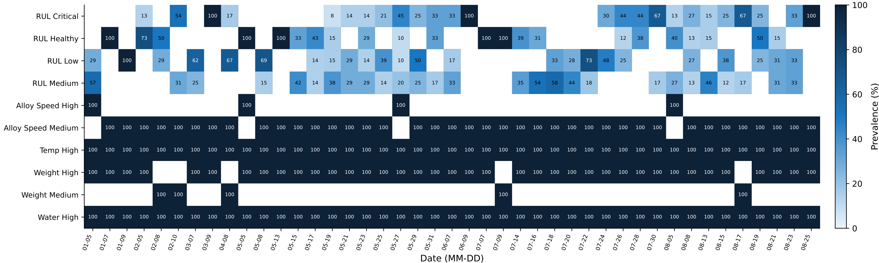
Figure 1 - Attribute Prevalence Heatmap (% concepts per day)
