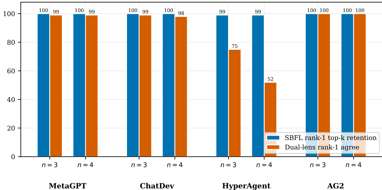
Bootstrap frequency (%)
