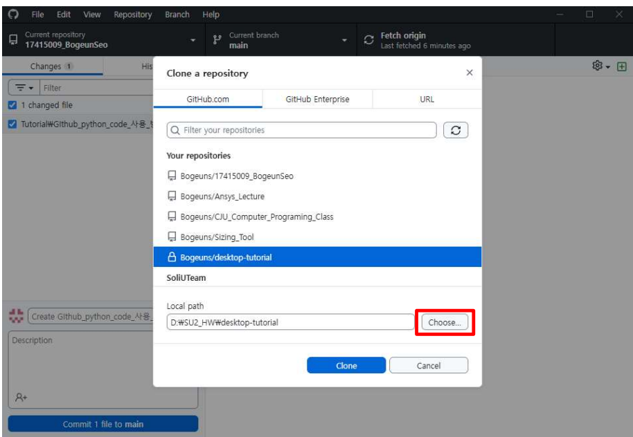
Fig. 3 Repository Clone
