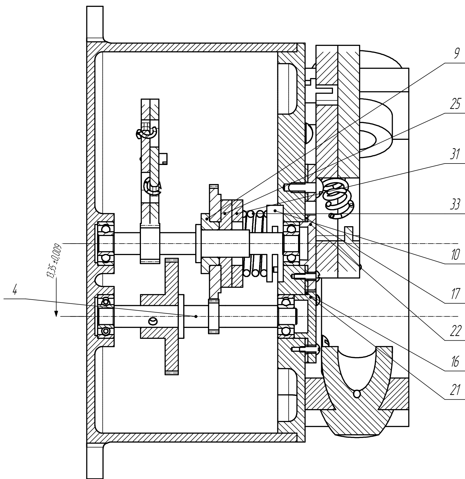
В-В (2,5:1)
