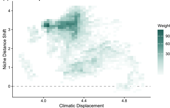
(a) Climatic Displacement vs Niche Distance Shift
