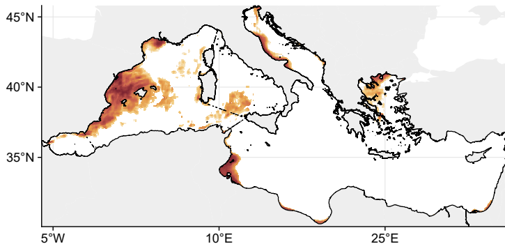
(b) Positive Niche Distance Shift: Pareto depth
