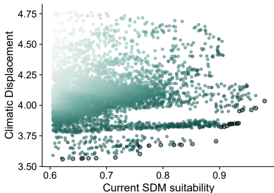
(c) Low Climatic Displacement: decision plane
